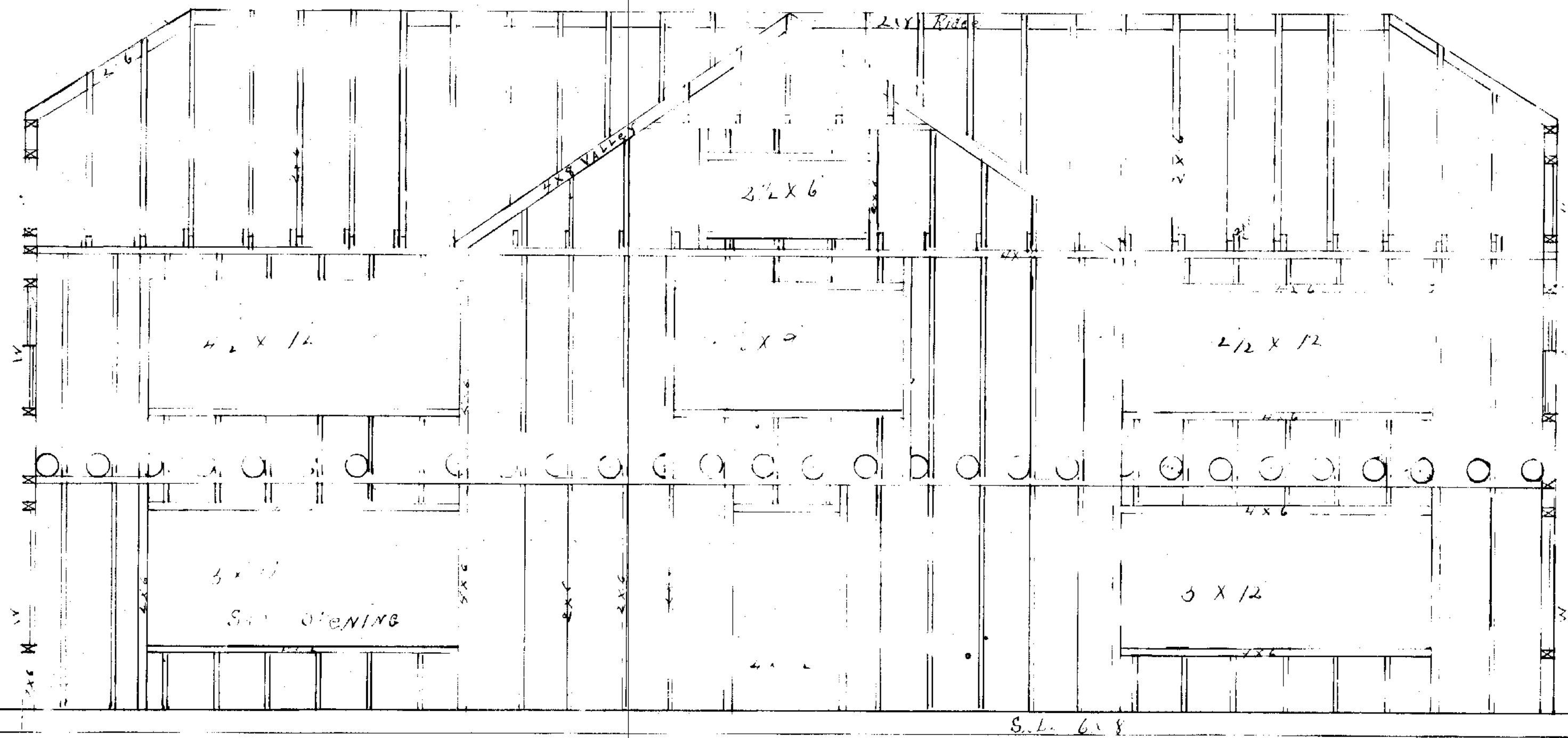
Front Elevation of Frame Showing Size and Location of Timbers Plan Made By G.H. Rogers North River N.Y. for Thomas S. Walker
