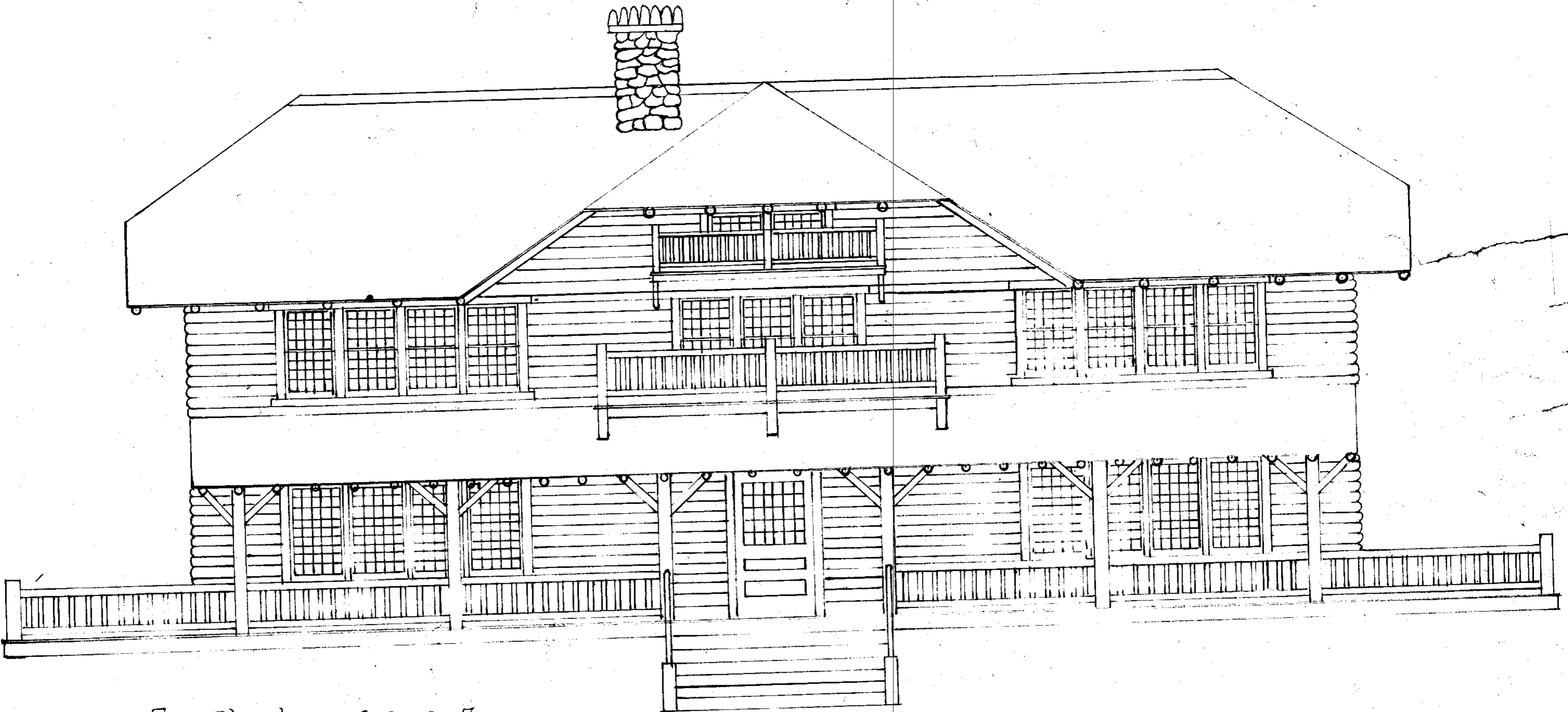
Front Elevation of CAMP for THOMAS S WALKER At LONG LAKE N.Y. PLANS MADE BY C.H. ROGERS North River N.Y.
