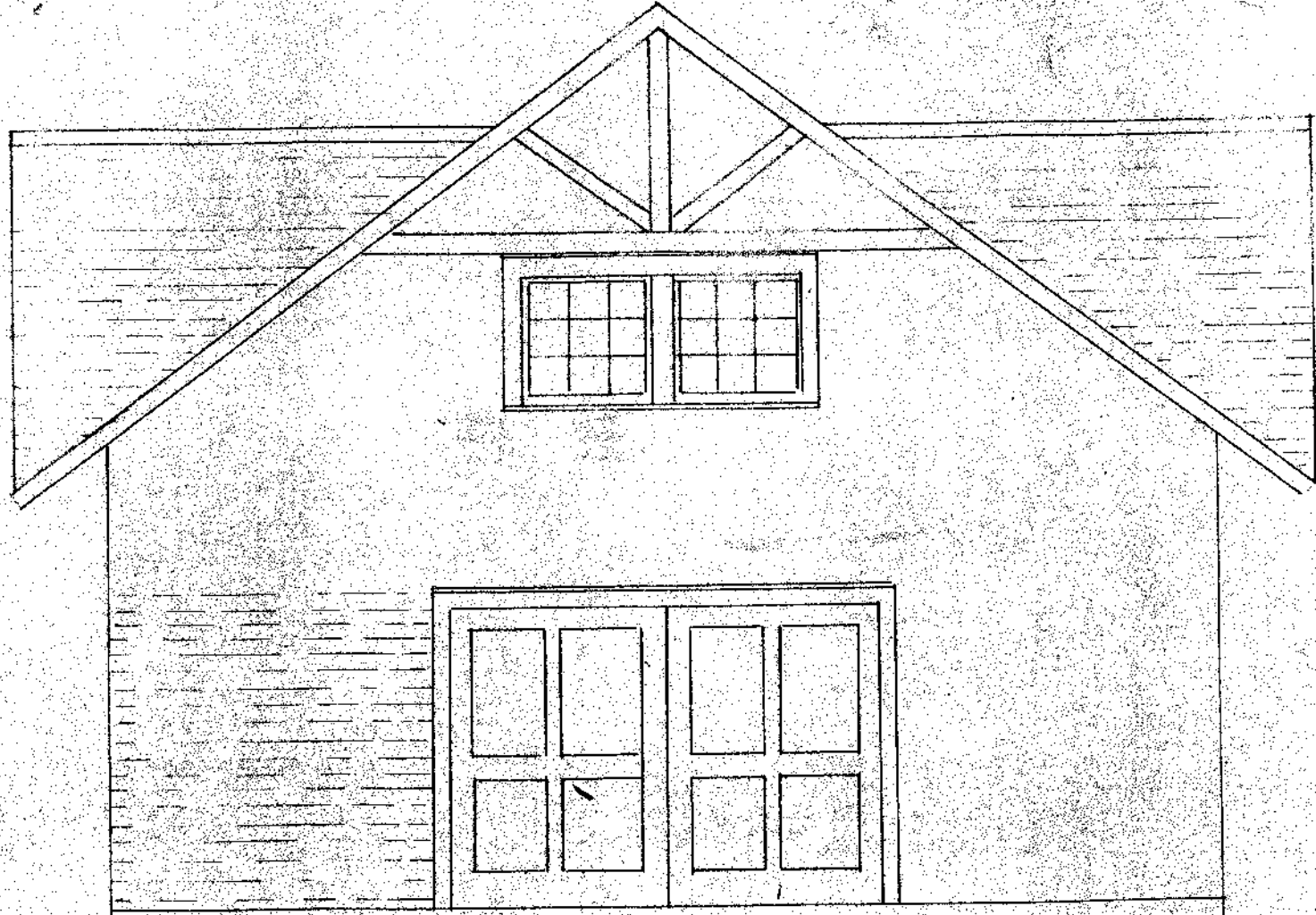
FRONT ELEVATION OF BOAT HOUSE FOR THOMAS S. WALKER AT LONG LAKE N.Y. CH. ROGERS ARCHITECT NORTH RIVER N.Y. SCALE 1/4" TO 1'-0"
