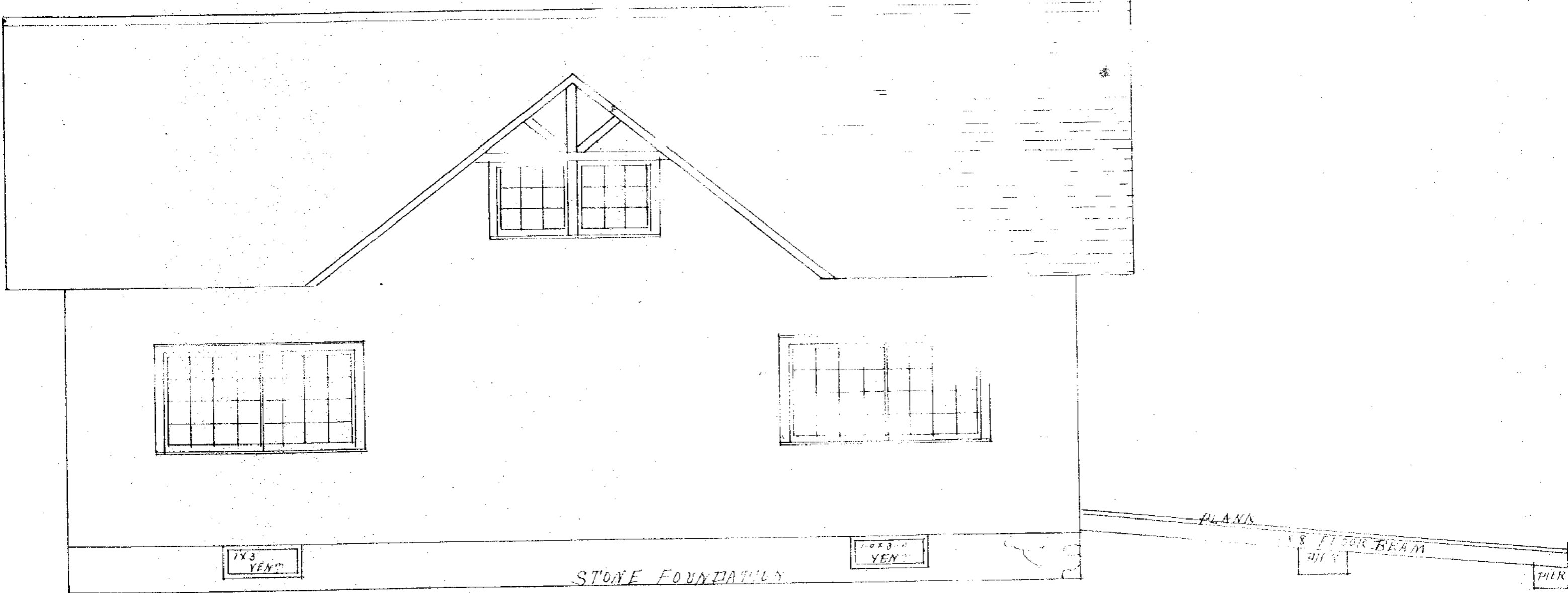
LEFT SIDE ELEVATION OF BOAT HOUSE FOR THOMAS S WALKER AT LONG LAKE NY G. H. ROGERS ARCHITECT NORTH RIVER N.Y. SCALE 1/4" TO 1'-0"
